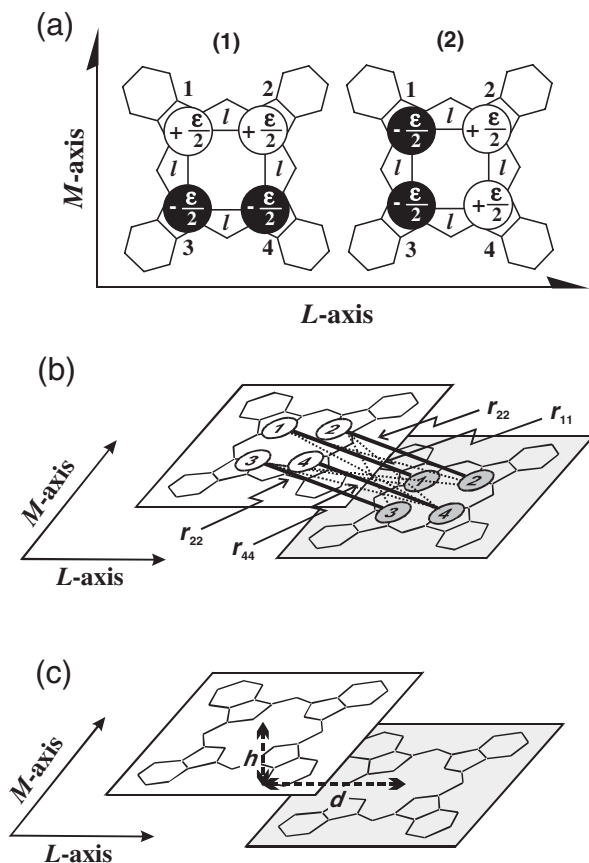
Fig. 6. (a) Extended double-dipole (EDD) model of Pc molecule of Sakakibara et al. 42 Each four charges ( \pm \epsilon/2 ) are located at the corners of Pc molecular plane separated by a distance l . The total moment exists along the M -axis in (1), and it exists along the L -axis in (2). (b) r_{ab} ( a or b = 1-4 ) are distances between charges located on different molecules. (c) The interplane distance ( h ) and slipping distance ( d ) are sketched.
