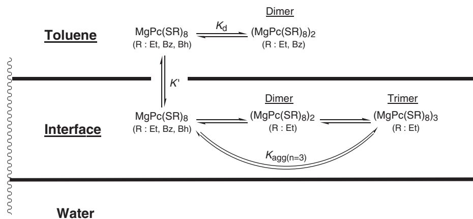
Scheme 2. Proposed scheme for the interfacial adsorption and aggregation mechanism of \text{MgPc}(\text{SR})_8 derivatives in the toluene/water system.
