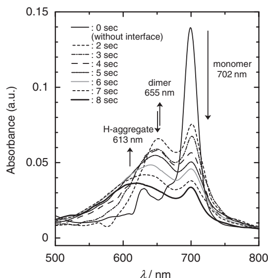
Fig. 4. The spectral change due to the interfacial aggregation of \text{MgPc(SET)}_8 at the toluene/water interface measured by CLM technique. The absorption spectra were recorded at 1 s intervals until the adsorption equilibrium was achieved (8 s). The concentration of \text{MgPc(SET)}_8 was 1.0 \times 10^{-6} M. The arrows indicate the direction of the spectral changes with the time course.
