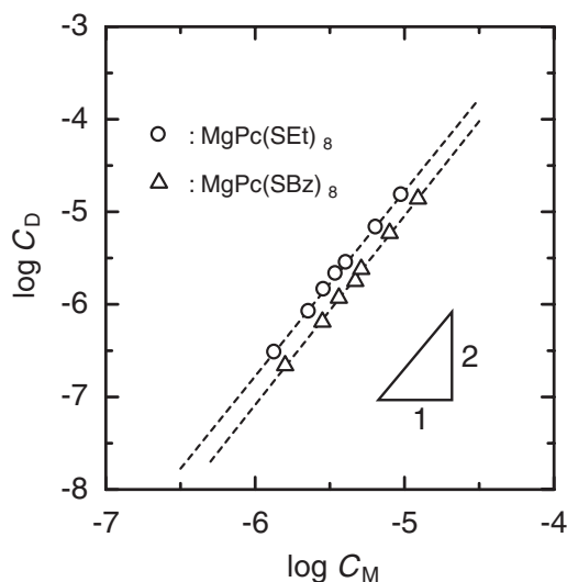
Fig. 2. Plots of \log C_D vs \log C_M for \text{MgPc}(\text{SET})_8 (open circle) and \text{MgPc}(\text{SBz})_8 (open triangle) in toluene. The broken lines are the least-squares fitted ones, which slopes were close to 2. The correlation coefficient was larger than 0.99 for both plots.
