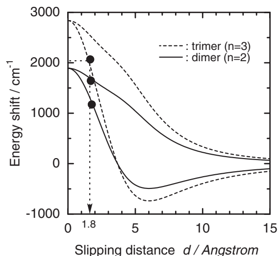
Fig. 7. The EDD model simulation of energy shift (cm -1 ) of the two absorption bands shown as a function of slipping distance (Å). The interplane distance ( h ) and the dipole length ( l ) are fixed at 3.26 Å and 4 Å, respectively. The upper lines correspond to M - M components and the lower lines correspond to L - L components. n is the number of Pc molecules.
