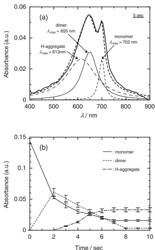
Fig. 5. (a) Example of deconvolution analysis; (b) time profile of the maximum absorbances of monomer, dimer, and H-aggregate.
