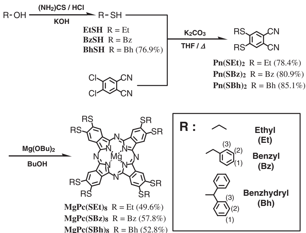
Scheme 1. Reaction routes for the syntheses of phthalocyaninatomagnesium(II) with eight peripheral thioether substituents.
