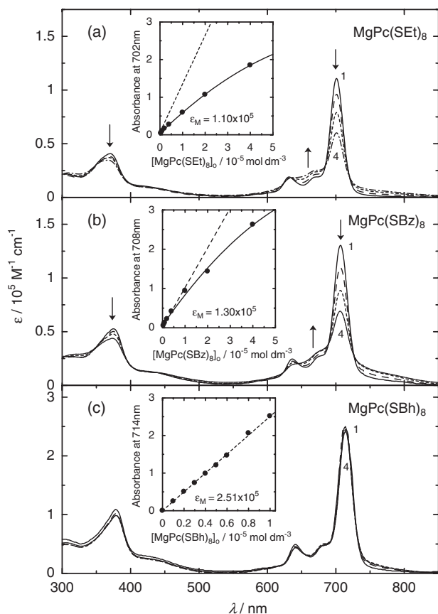
Fig. 1. Concentration dependence of absorption spectrum of \text{MgPc}(\text{SR})_8 derivatives in toluene (top: \text{MgPc}(\text{SET})_8 , medium: \text{MgPc}(\text{SBz})_8 , bottom: \text{MgPc}(\text{SBh})_8 ): 1) 1.0 \times 10^{-6} \text{ mol/dm}^3 ; 2) 5.0 \times 10^{-6} \text{ mol/dm}^3 ; 3) 1.0 \times 10^{-5} \text{ mol/dm}^3 ; 4) 2.0 \times 10^{-5} \text{ mol/dm}^3 . The insets show Lambert-Beer law plots for the absorbance at Q band of \text{MgPc}(\text{SR})_8 monomer; the slopes of broken lines gave molar absorptivities of monomers, \epsilon_M . The arrows indicate the direction of the absorbance changes with increasing concentration.
